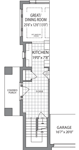
PARTIAL MAIN LEVEL ELEVATION C
