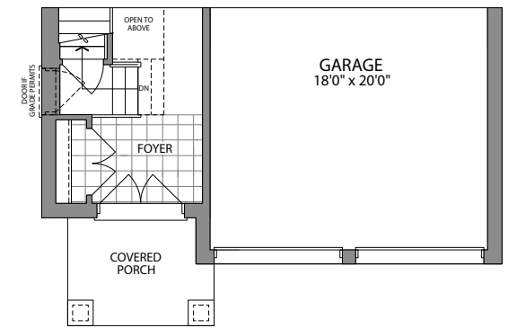
PARTIAL MAIN LEVEL ELEVATION B & C
