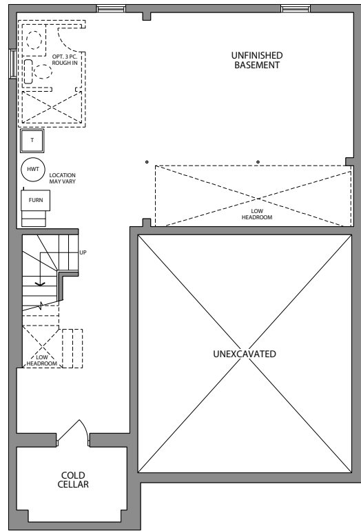
LOWER LEVEL ELEVATION A
