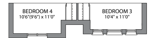
PARTIAL UPPER LEVEL ELEVATION C
