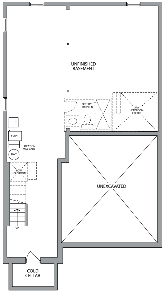
LOWER LEVEL ELEVATION C
