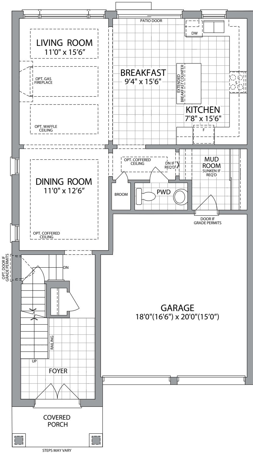
MAIN LEVEL ELEVATION A
