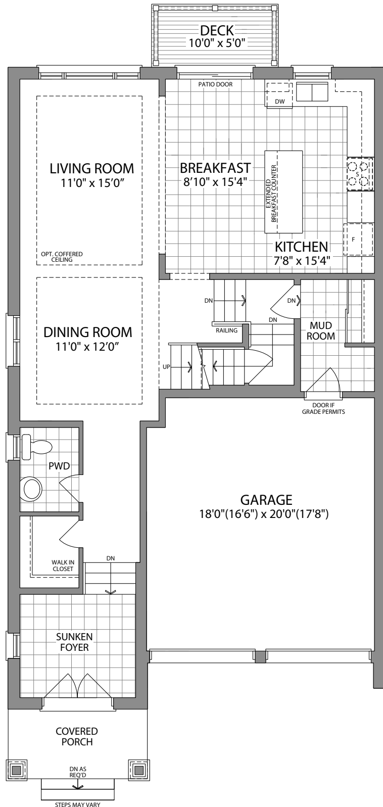
MAIN LEVEL ELEVATION C
