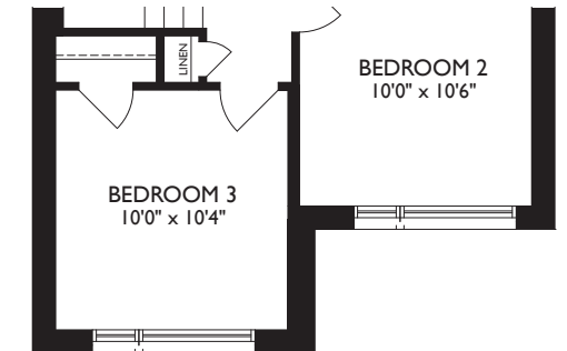
PART. UPPER LEVEL - ELEV. C SIMILAR TO ELEV. B
