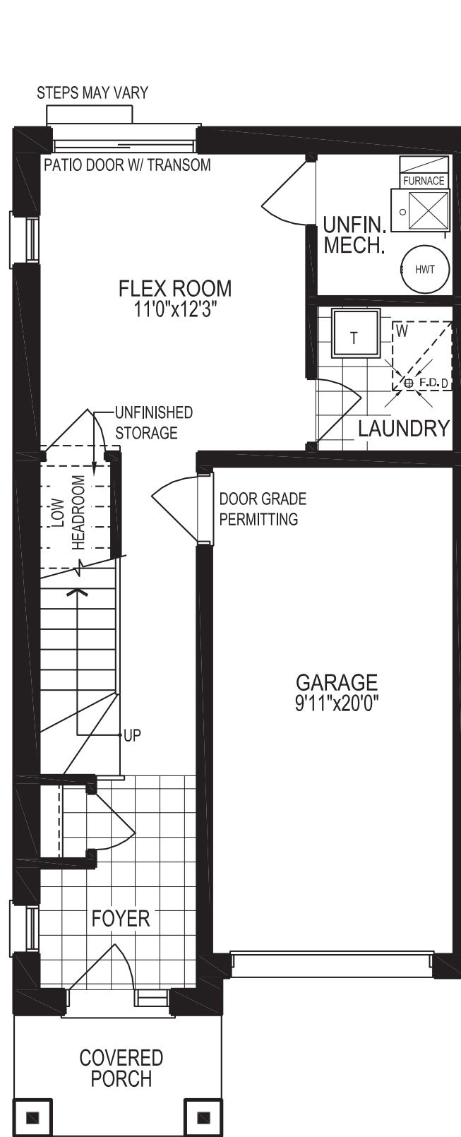
LOWER LEVEL ELEV. A
