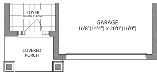
PARTIAL MAIN LEVEL ELEVATION A & C
