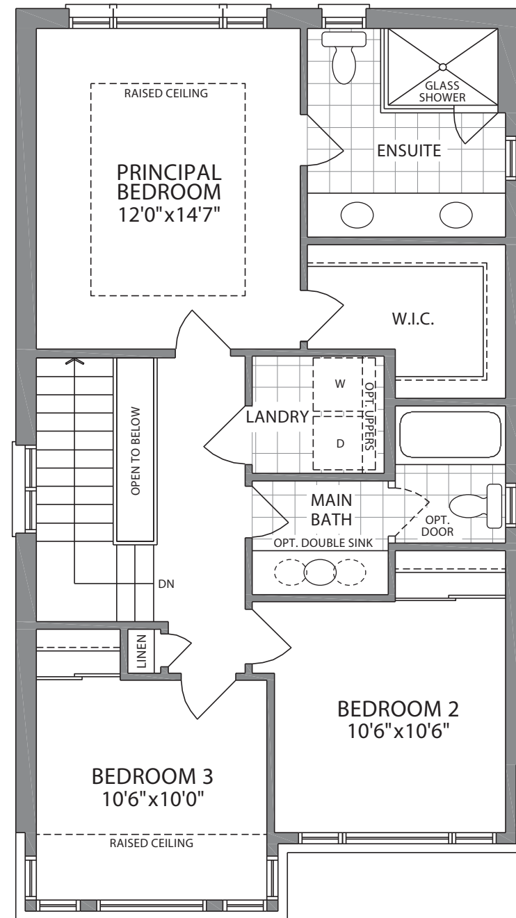
UPPER LEVEL ELEVATION B
