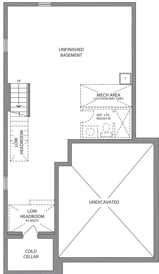
LOWER LEVEL ELEVATION A, B, & C
